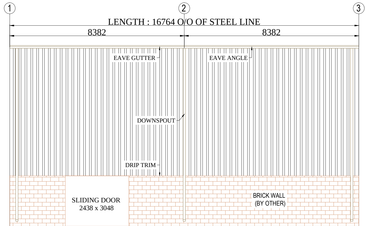
SIDE WALL SHEETING
