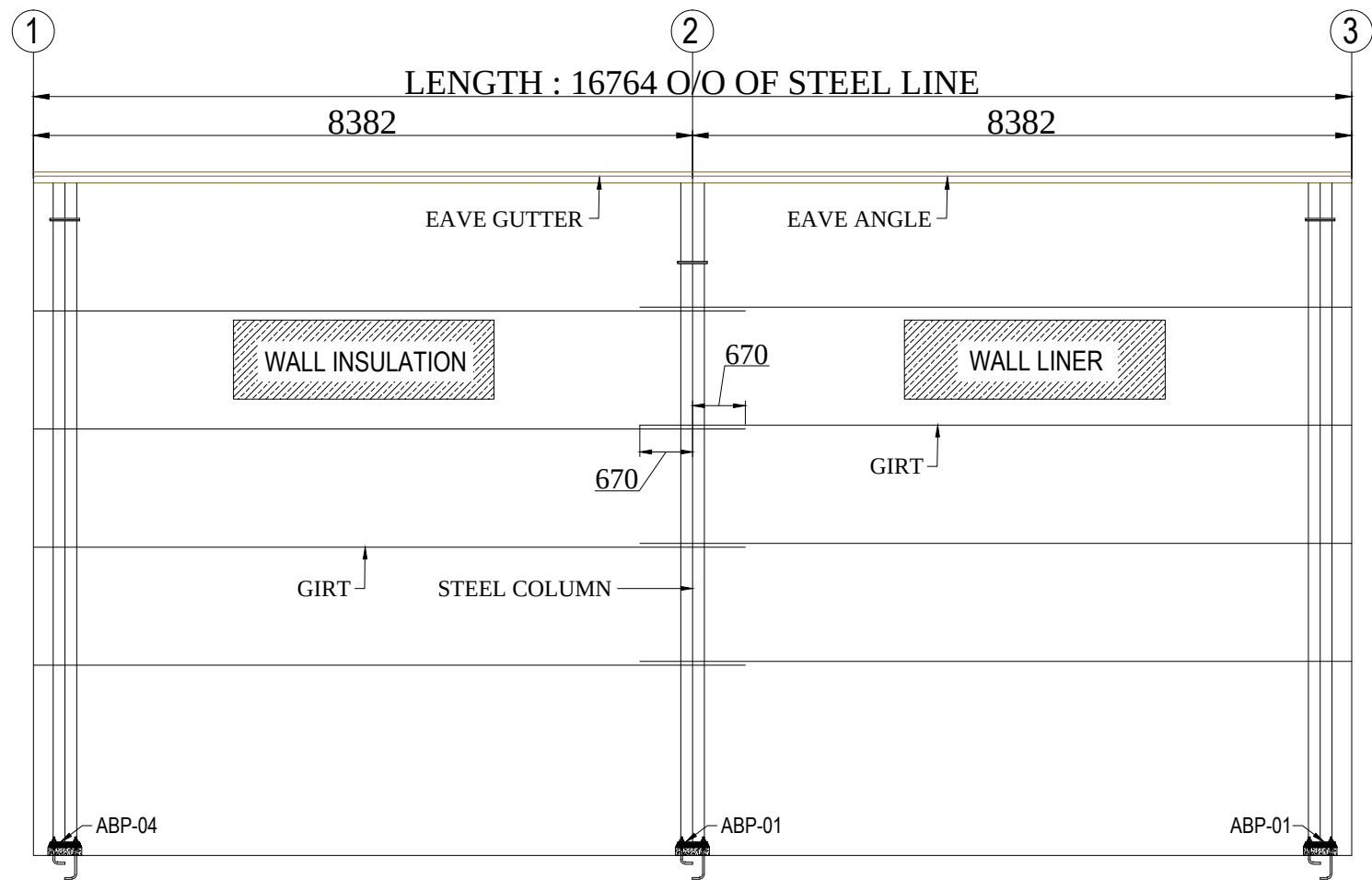
SIDE WALL FRAMING
